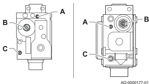
Abb.45 Gasarmaturen
